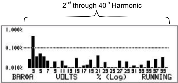
Figure 42. Harmonics Bargraph \Phi A, VOLTS % Log display
