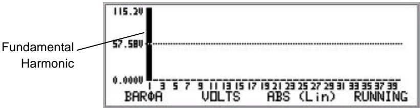
Figure 43. Harmonics \Phi A VOLTS ABS Lin display
