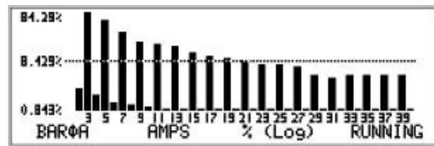
Figure 46. Harmonics Bargraph \bar{A} , AMPS % Log display
