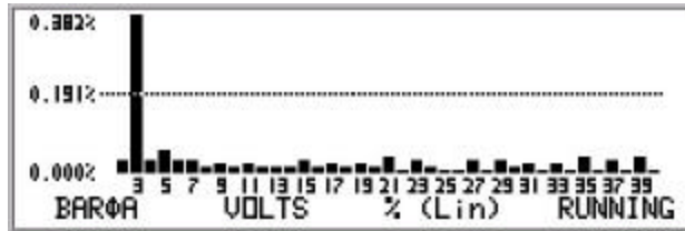
Figure 45. Harmonics Bargraph \bar{A} , VOLTS % Lin display
