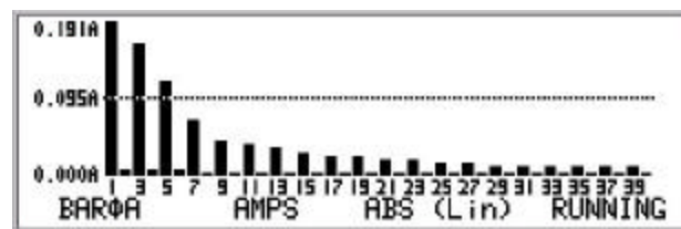
Figure 47. Harmonics Bargraph \bar{A} , AMPS ABS Lin display
