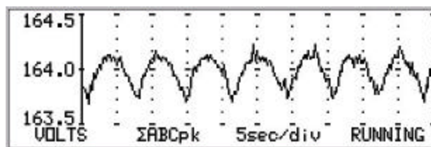
Figure 63. History VOLTS \hat{a}ABC PEAK display
