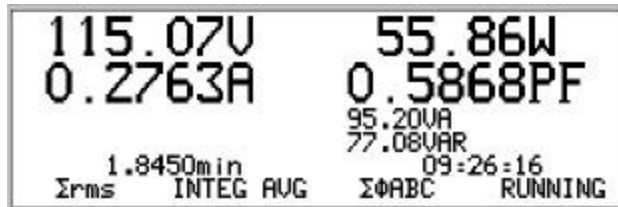
Figure 29. Basics \hat{r}MS INTEG AVG \hat{f}ABC display
