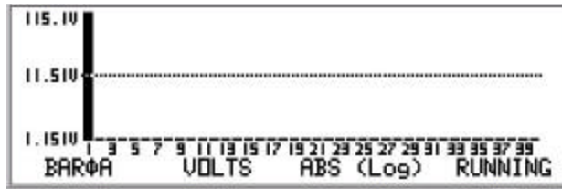
Figure 44. Harmonics Bargraph \bar{A} , VOLTS ABS Log display
