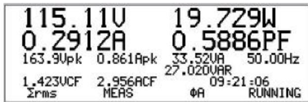
Figure 18. Basic \hat{a}RMS sample display
