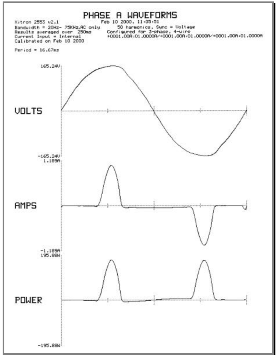
Figure 83. Phase A Waveforms graphic printout
